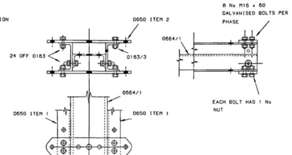
ENLARGED DETAIL A SCALE 1:7.5
