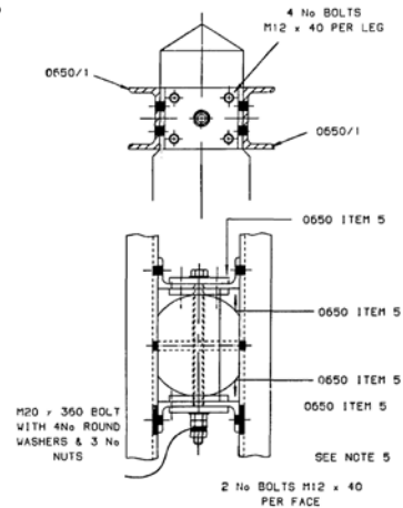
ENLARGED DETAIL OF CROSSARM FIXING SCALE 1:7.5
